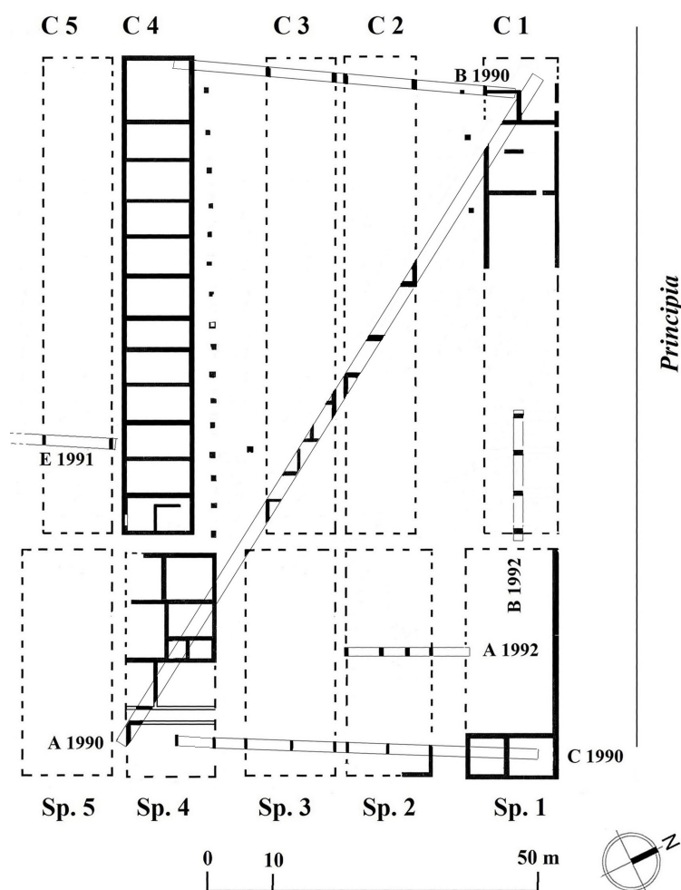
Figure 7. Cohors miliaria. Plan.
